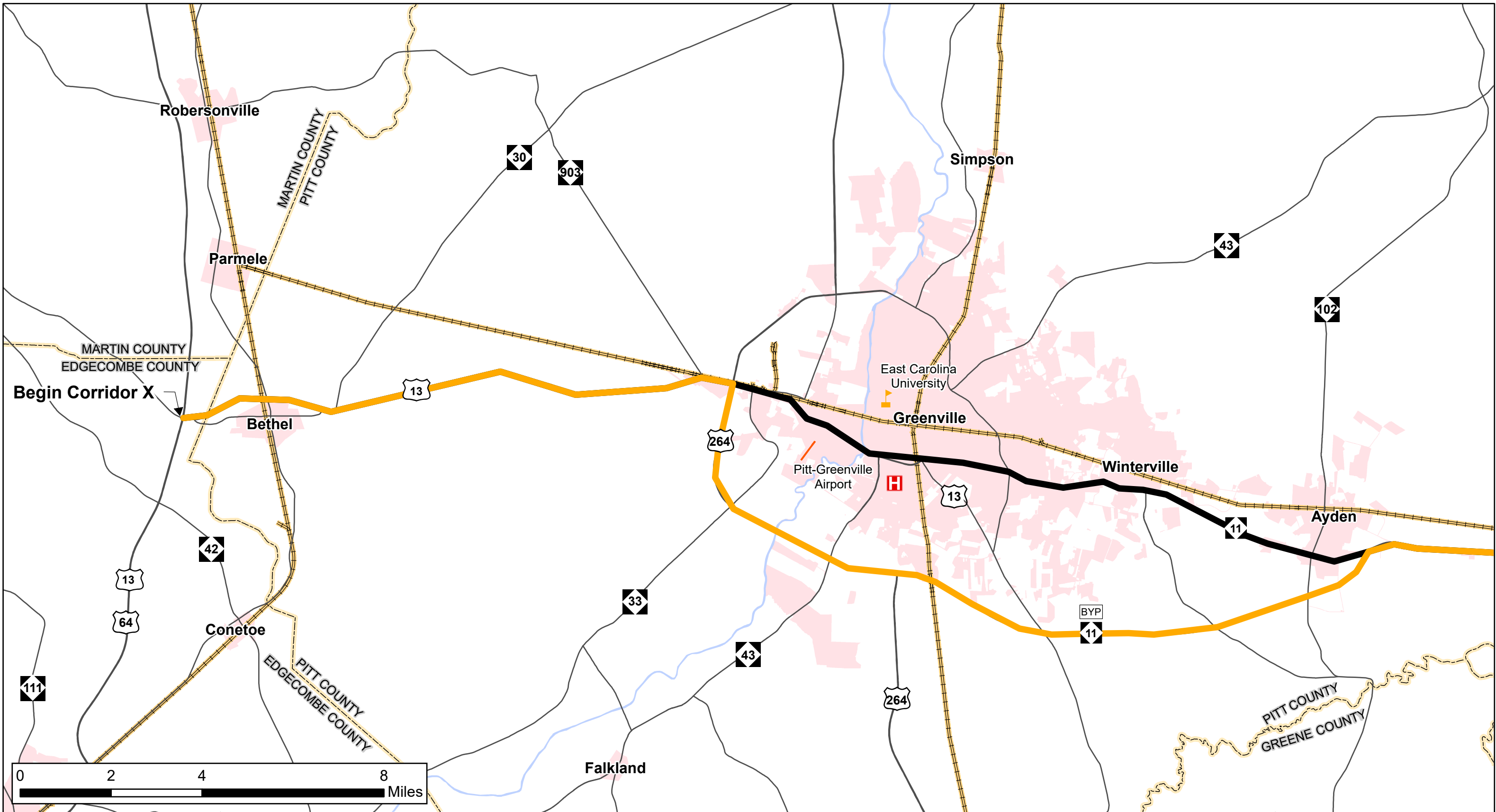
CORRIDOR X ALIGNMENT U.S. 13/U.S. 264/N.C. 11/ C.F. Harvey Pkwy/U.S. 258 FIGURE 3A: US 13 TO GREENVILLE
